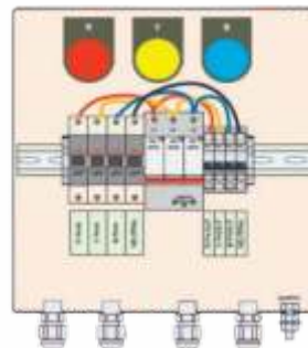
THREE PHASE ACDB
