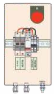
SINGLE PHASE ACDB
